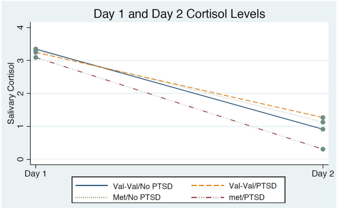
Figure 4. n = 173; Note: Salivary cortisol is given in [\log(\mu\text{g/dL}) \times 100] ; circles represent mean salivary cortisol levels; this model included the following covariates: age, race, years of education, adult trauma exposure, % dexamethasone suppression, and a female x child abuse interaction term.
